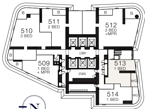
TOWER 1 - LEVEL 5
